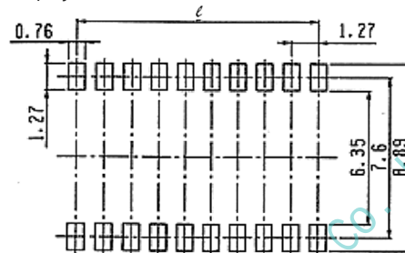
PCB DIMENSION
